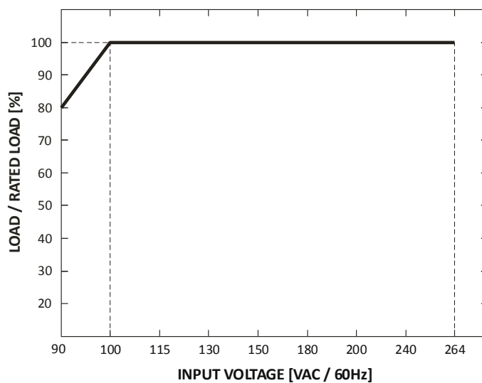
STATIC CHARACTERISTIC
