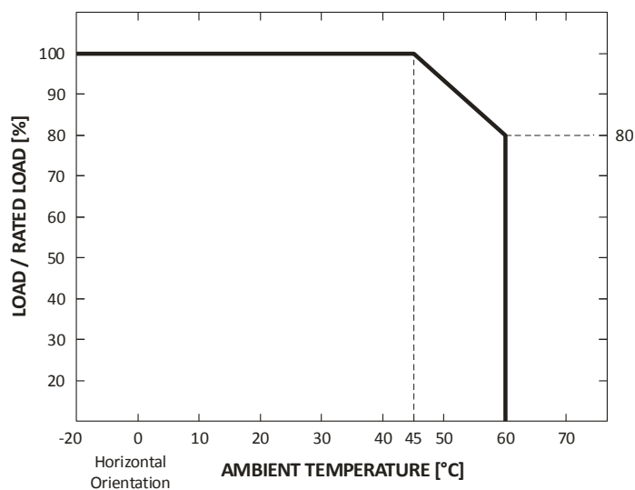
DERATING CURVE
