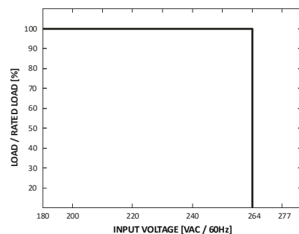
STATIC CHARACTERISTIC
