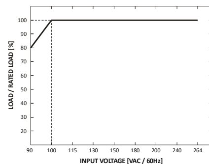
STATIC CHARACTERISTICS
